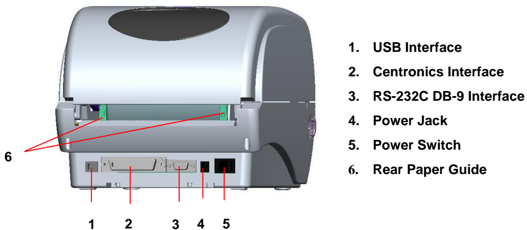
Fig. 2 Rear view
